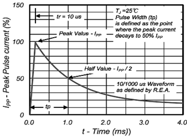
Fig 2: Pulse Waveform
