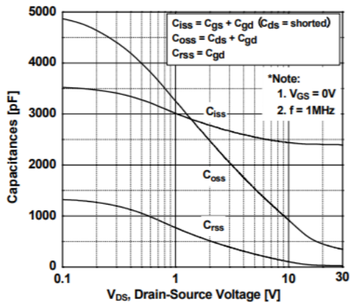
Figure 5. Capacitance Characteristics
