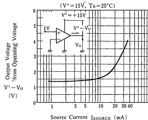
Source Current
