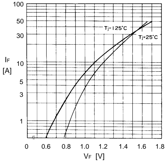
Forward characteristics
