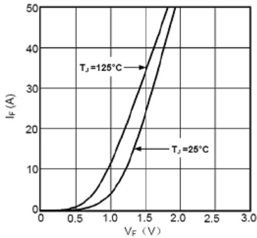
Fig1. Forward Voltage Drop vs Forward Current
