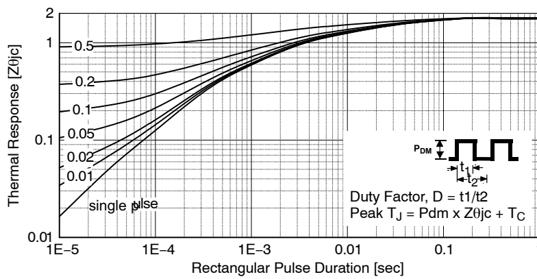
Figure 26. Transient Thermal Impedance of Diode
