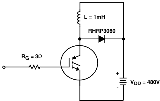
FIGURE 17. INDUCTIVE SWITCHING TEST CIRCUIT
