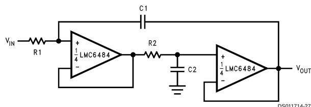
FIGURE 25. Rail-to-Rail Single Supply Low Pass Filter
