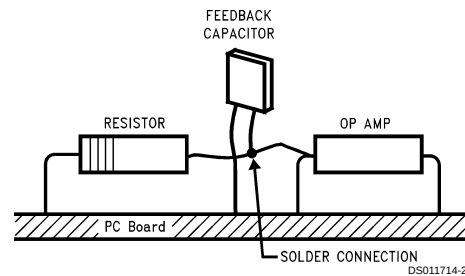
FIGURE 11. Air Wiring
