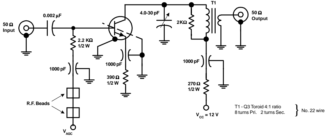
FIGURE 1: 45 MHz Power Gain Circuit
