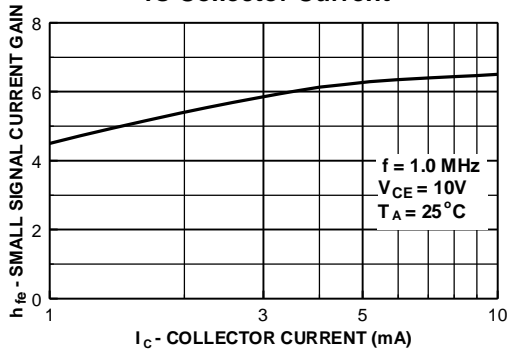
Small Signal Current Gain vs Collector Current
