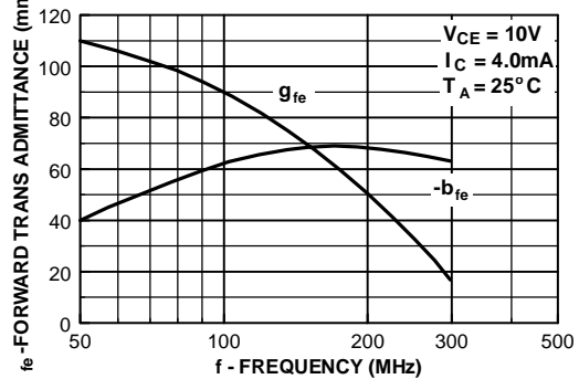
Forward Transfer Admittance vs Frequency
