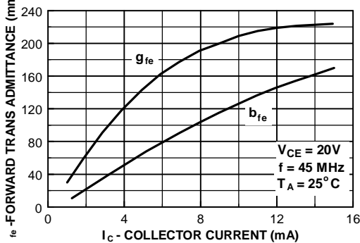
Forward Transfer Admittance vs Collector Current
