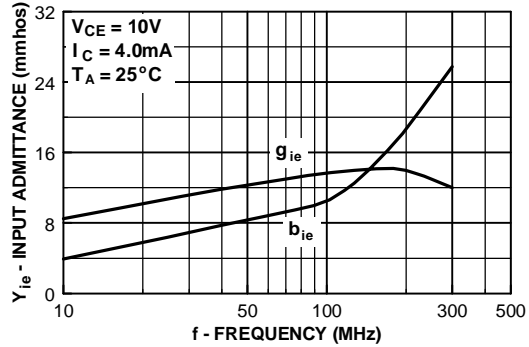
Input Admittance vs Frequency
