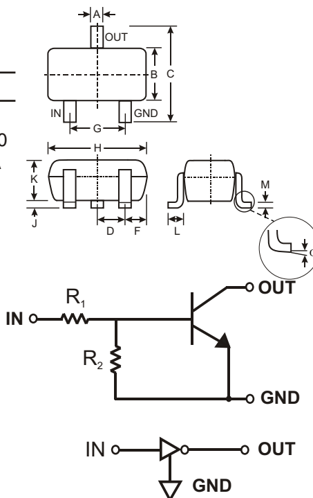
SCHEMATIC DIAGRAM
