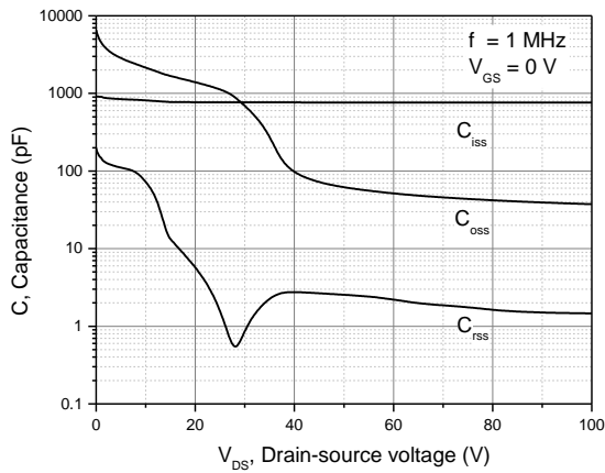
Figure 3. Typ. capacitances
