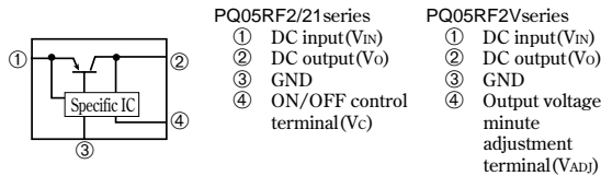
Internal connection diagram
