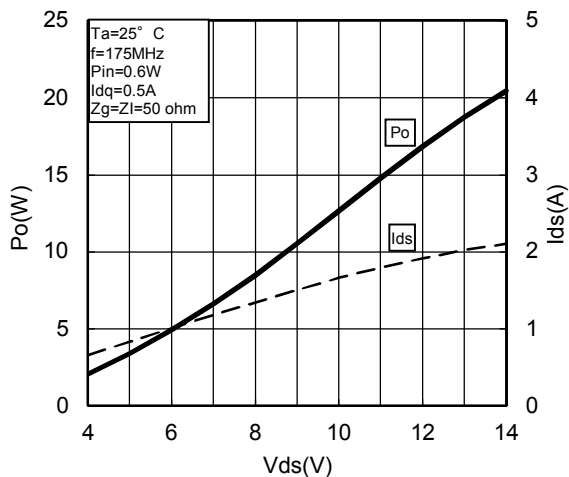
Vds-Po CHARACTERISTICS
