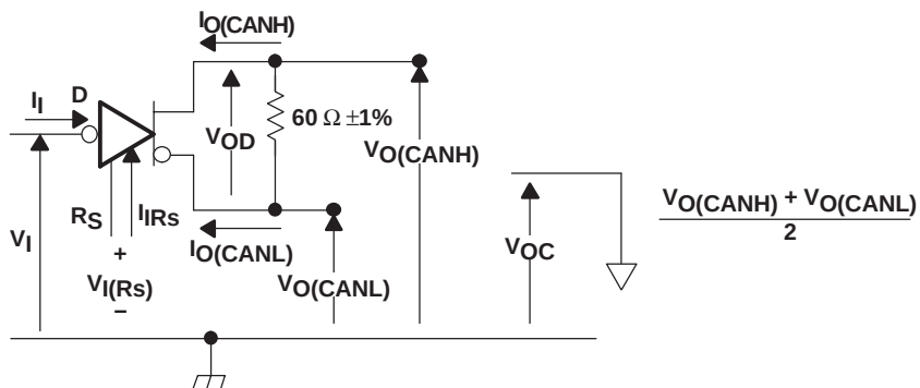
Figure 1. Driver Voltage, Current, and Test Definition
