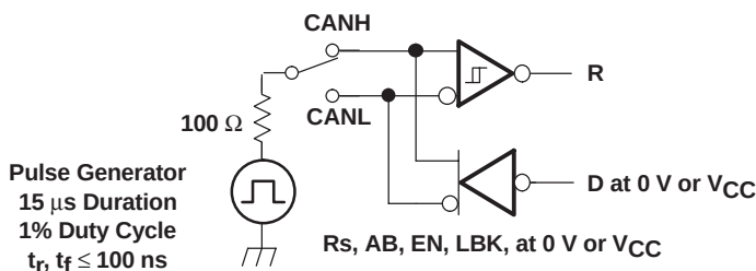
INPUT OUTPUT MEASURED V CANH V CANL R |V id | -6.1 V -7 V L V OL 900 mV 12 V 11.1 V L 900 mV -1 V -7 V L 6 V 12 V 6 V L 6 V -6.5 V -7 V H V OH 500 mV 12 V 11.5 V H 500 mV -7 V -1 V H 6 V 6 V 12 V H 6 V open open H X
